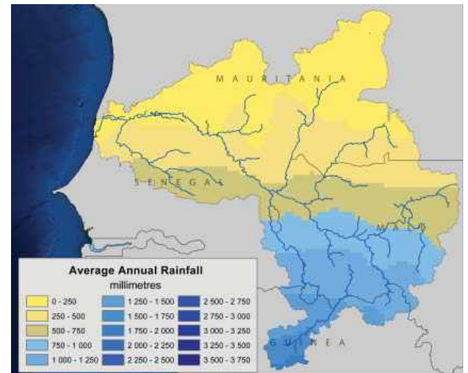
Figure 2.12.2: Senegal Basin average annual rainfall
