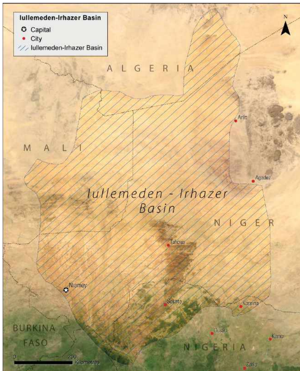
Figure 2.18.1: Iullemeden-Irhazer Basin
