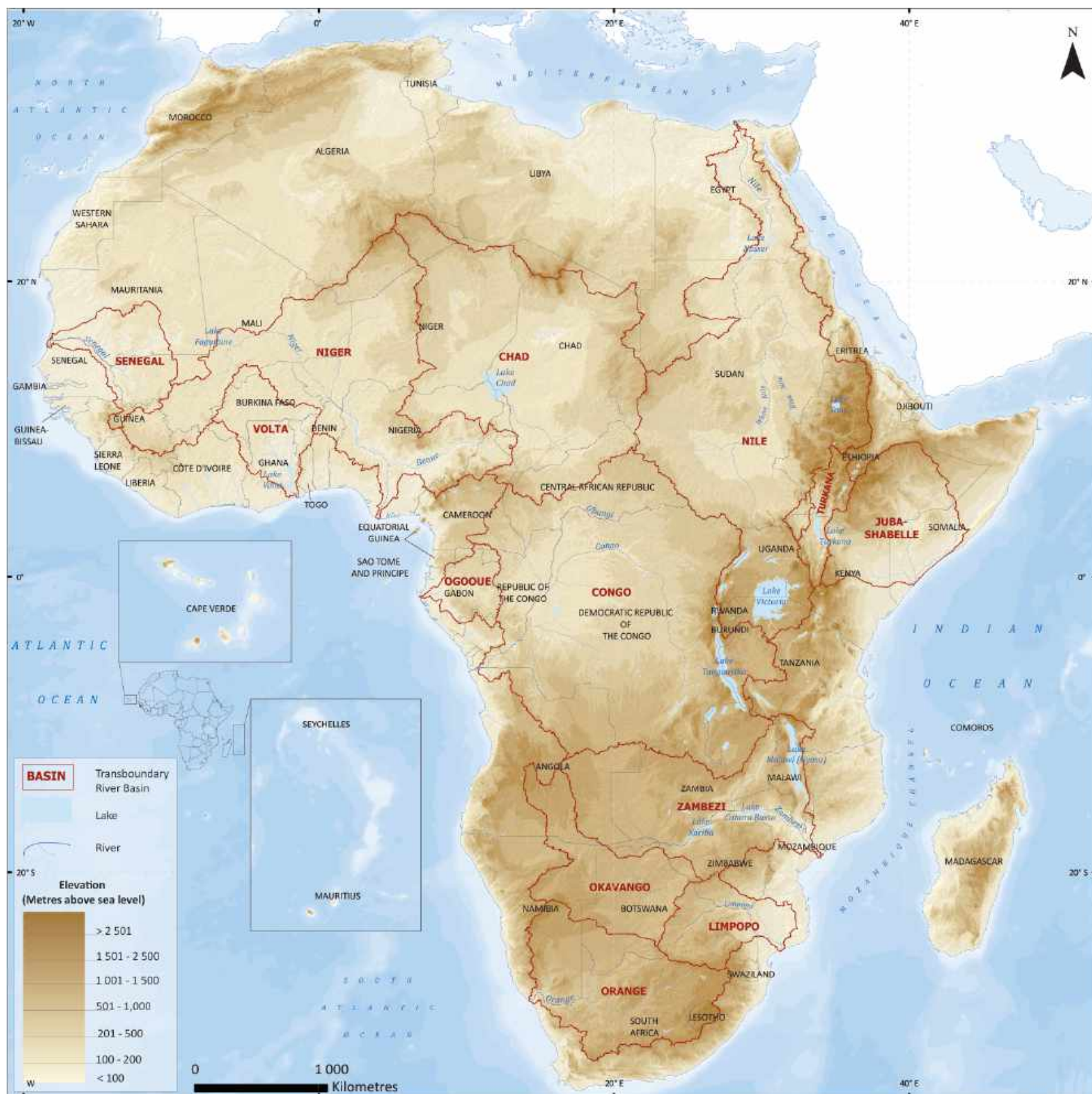
Figure 2.1: Africa's major transboundary river basins
